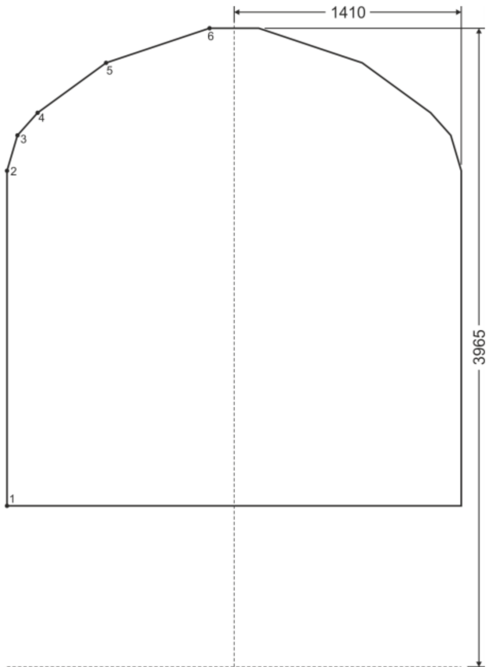
Figure D.1 W6a upper gauge diagram
